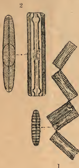
Fig. 332. — 1. Diatoma vulgare , Bory. 2. Grammatophora marina .
